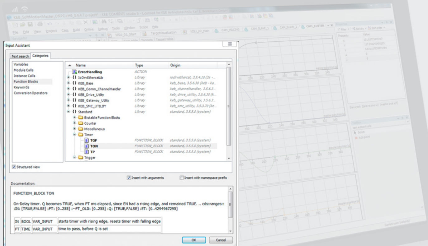
Input assistant
