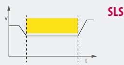
Safely-Limited Speed
